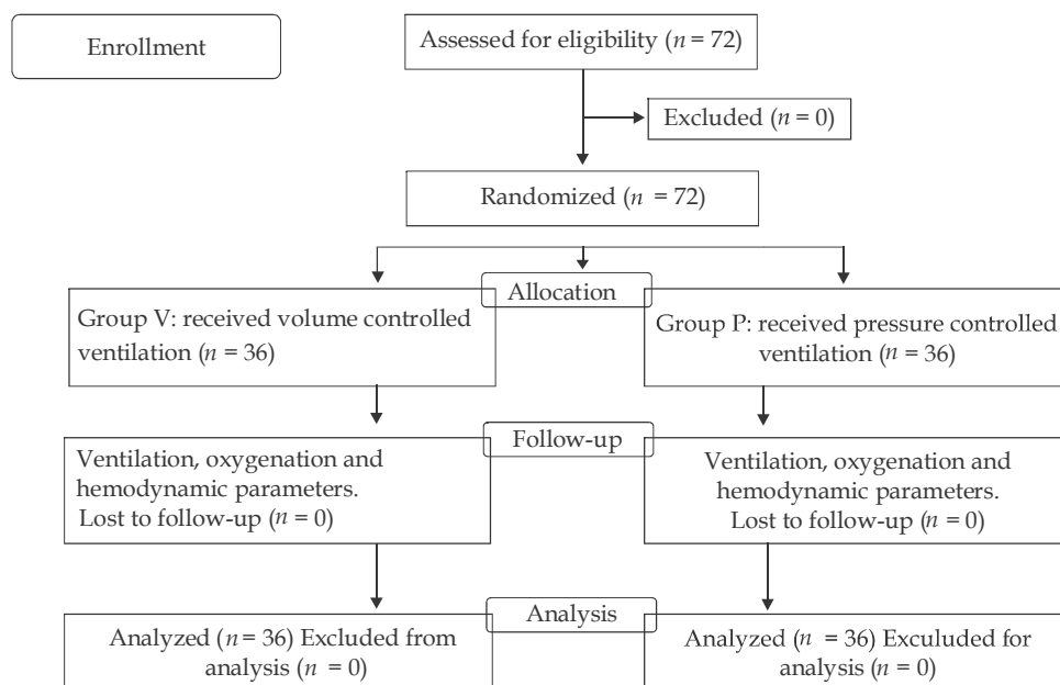
Fig. 1: Consort diagram
